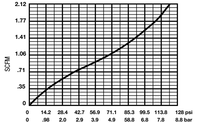
Diagram 1 Venting Capacity
